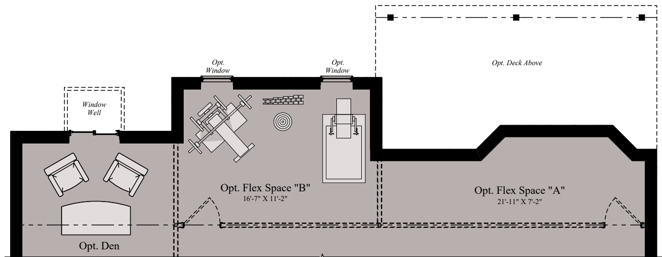
PARTIAL LOWER LEVEL - W/ OPT. SUNROOM & OWNER SUITE EXTENSION - IN-GROUND CONDITION
