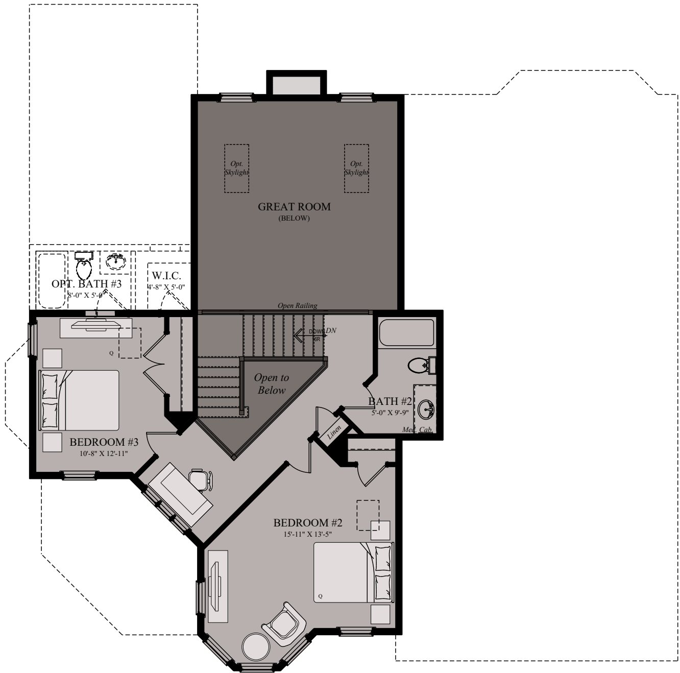
UPPER LEVEL - ELEVATION A
