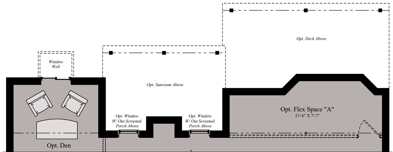
PARTIAL LOWER LEVEL - W/ OWNER SUITE EXTENSION IN-GROUND CONDITION
