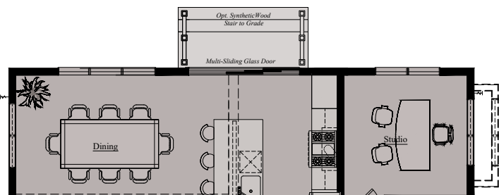
Main Level - Opt. Multi-Sliding Door + Opt. Stair to Grade
