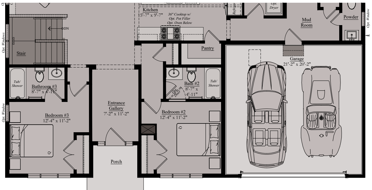
Partial Main Level - Opt. Bathroom #3
