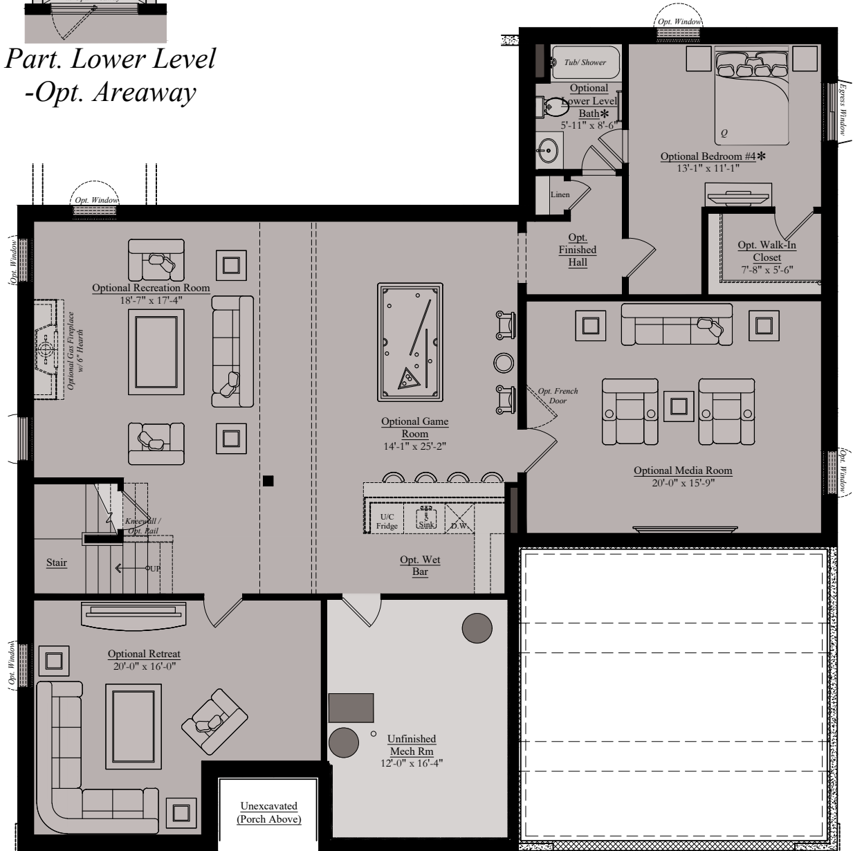
Lower Level - Opt. Rec. Rm., Opt. Game Rm., Opt. Bath, Opt. Bedroom, Opt. W.I.C., Opt. Retreat, Opt. Media Room, & Opt. Wet Bar
