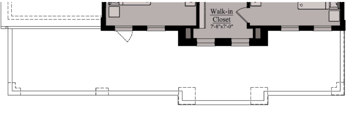
UPPER LEVEL - ELEV. 'C'
