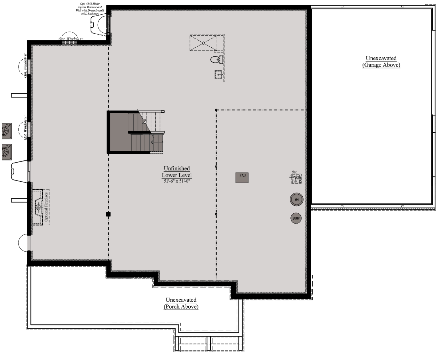
LOWER LEVEL - ELEV. 'A'
