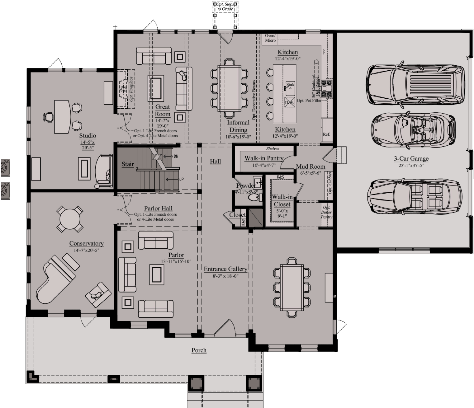
MAIN LEVEL - ELEV. 'A'
